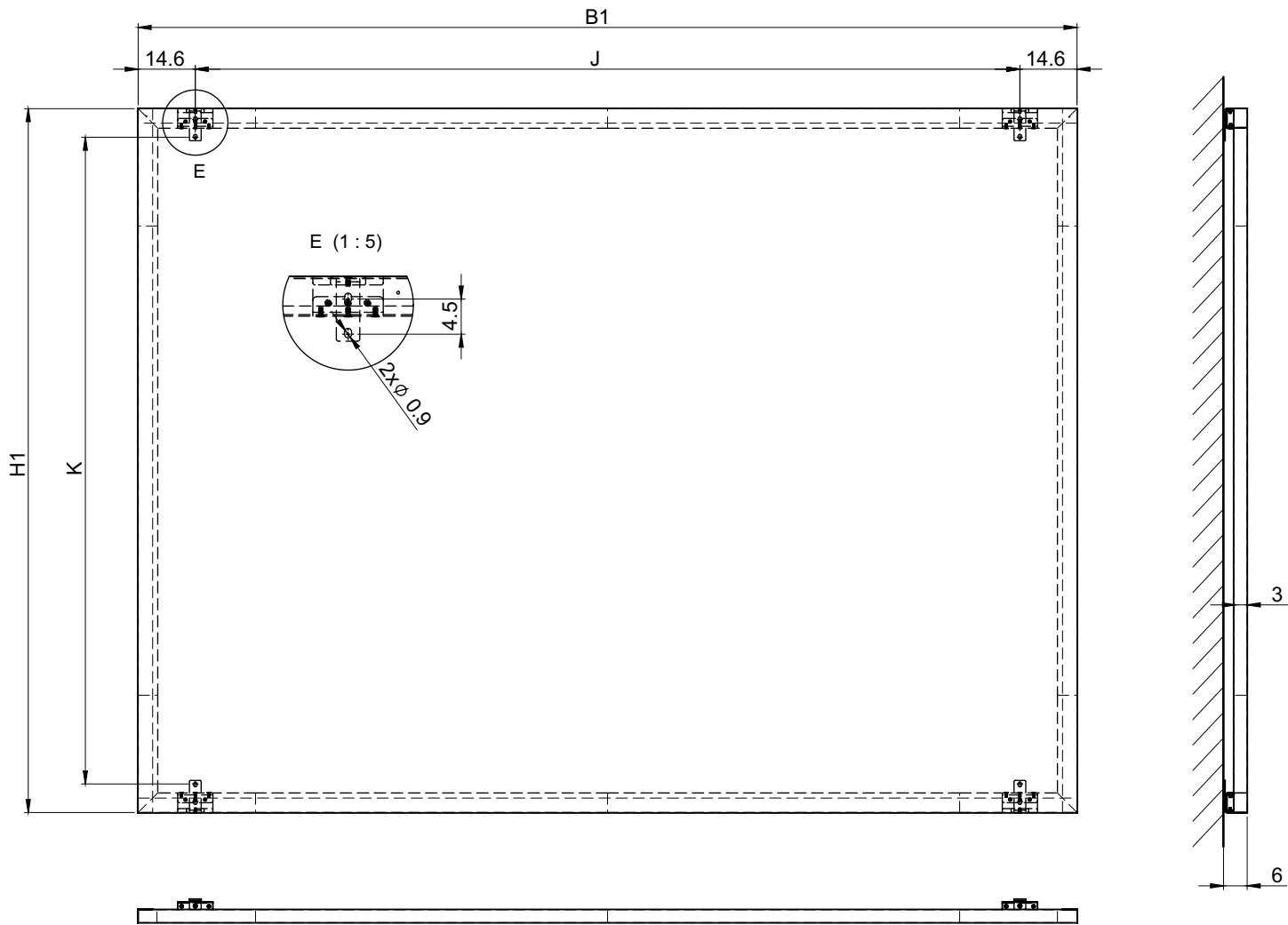
Dimensions in cm
